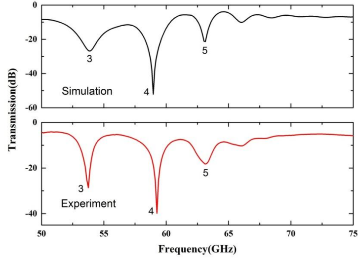
Fig. 12 Simulated and measured transmission coefficients S_{21} with CDR
