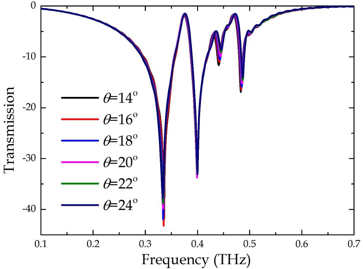
Fig. 8 transmission spectra at angles from 14^\circ to 24^\circ
