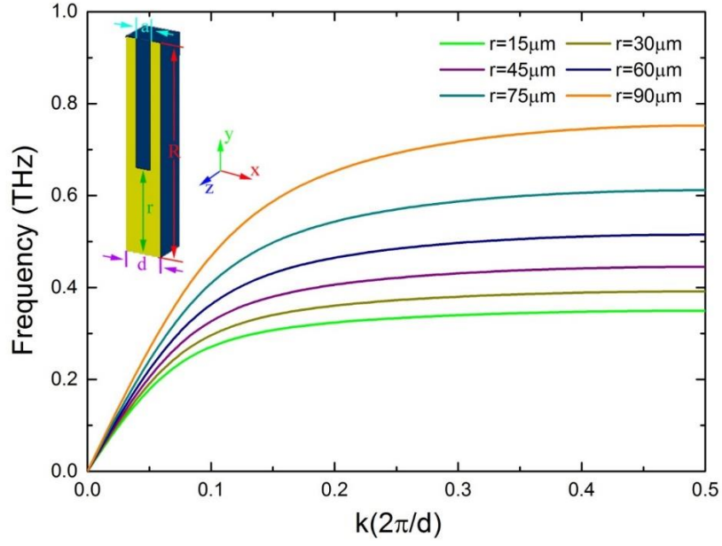
Fig. 2 Simulated dispersion curves of spoof LSPs for one periodic corrugated strips (see inset) with R = 150 \mu\text{m} , N = 36 , d = 2\pi R/N , a = 0.4d , and different lengths of r .
