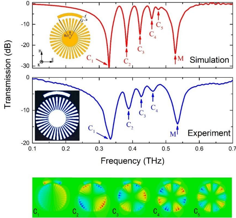
Fig. 1 theoretical and experimental transmission spectra of cap coupled corrugated texturing closed disk, bottom: electric field of multipolar resonances shown as dipole(C1), quadrupole(C2), hexapole(C3), octopole(C4), decapole(C5) mode. The resonance (M) comes from bright LSP mode supported by single CSR structure.
