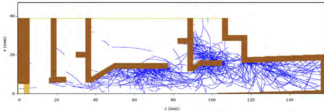
(c) Trajectories of the backscattered electrons.
