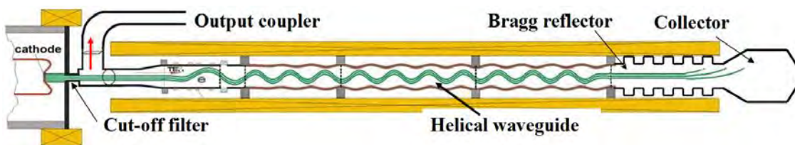
Fig. 2 The schematic of the W-band gyro-BWO.
