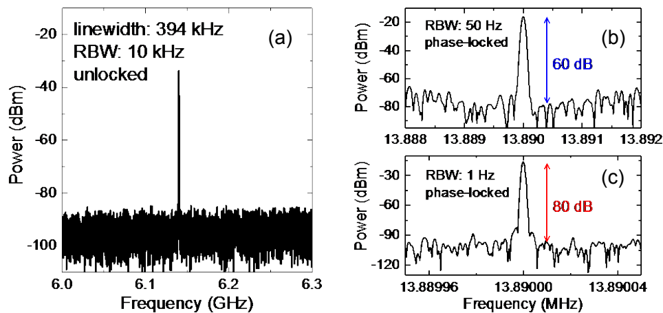
Fig. 4 IBN spectra of the free-running terahertz QCL comb (a), PLL-locked QCL measured with an RBW of 50 Hz (b) and 1 Hz (c).
