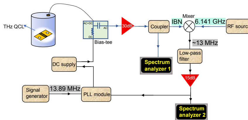
Fig. 3 Schematic plot of the PLL experimental setup.
