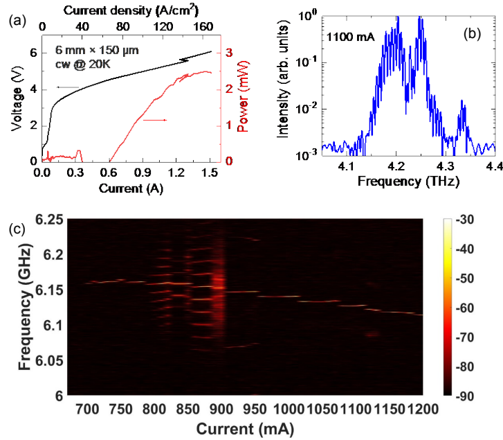
Fig. 2 Performance of the terahertz QCL. (a) Light-current-voltage characteristic of the 6-mm-long and 150- \mu m-wide laser in continuous wave mode measured at 20 K. (b) Normalized emission spectrum of the laser measured at 1100 mA at 20 K. (c) Inter-mode beat note mapping of the laser measured in the current range from 680 to 1200 mA.
