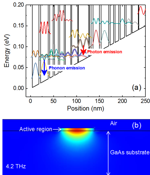
Fig. 1 Structure of active region and waveguide of QCL. (a) Sketch of conduction band structure, where the red arrow represents photon emission from bond state to continuum state and blue arrow represents phonon emission for fast carrier depletion. (b) Calculated electric field distribution of the laser with a single plasmon waveguide. The calculation was performed at a frequency of 4.2 THz.
